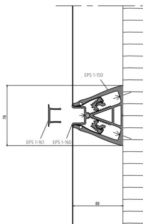
Attachement on wood
